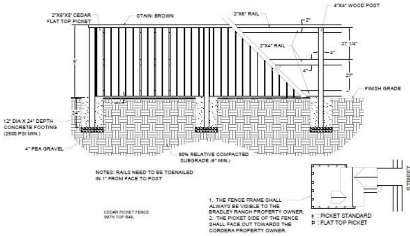
7 FENCE TYPE B: 5' CEDAR PICKET FENCE WITH TOP RAIL NTS
