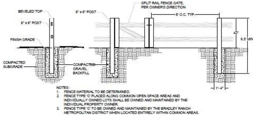
5 FENCE TYPE C: SPLIT RAIL FENCE DETAIL N.T.S.
